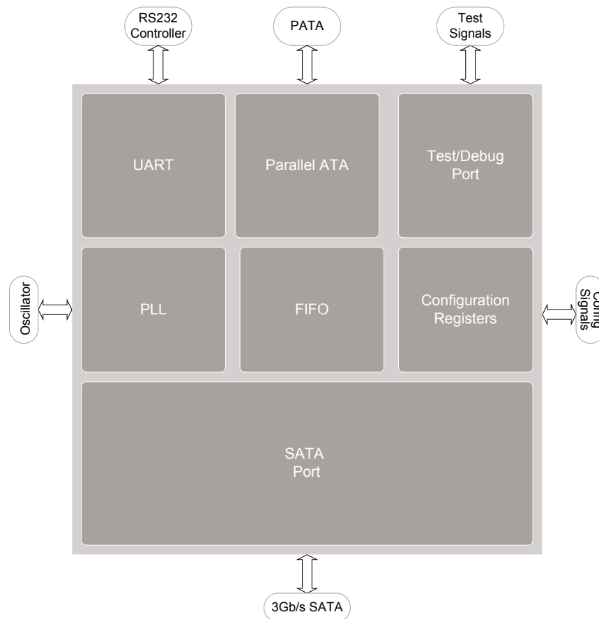
Fig 1. Marvell 88SA8052 PATA to SATA Bridge
