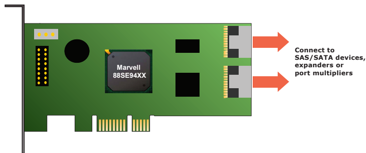
Fig 2. HBA (Host Bus Adapter) Application
