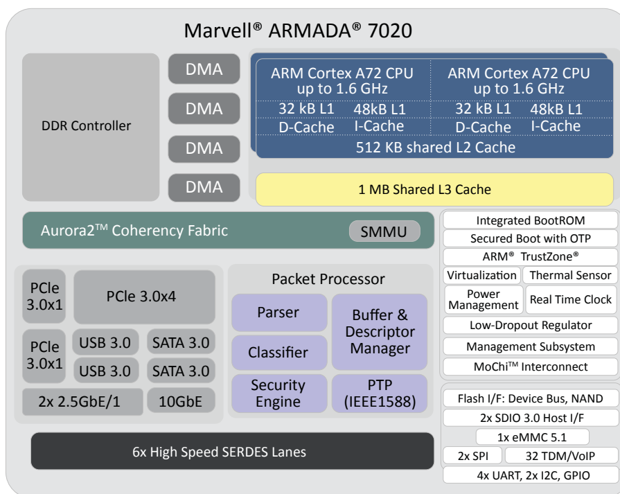
Marvell 88F7020 Quad-Core + MoChi Computing Platform
