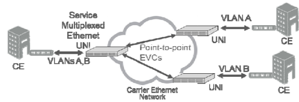
Figure 3. Ethernet Virtual Private Line (EVPL): VLAN-based service multiplexing
