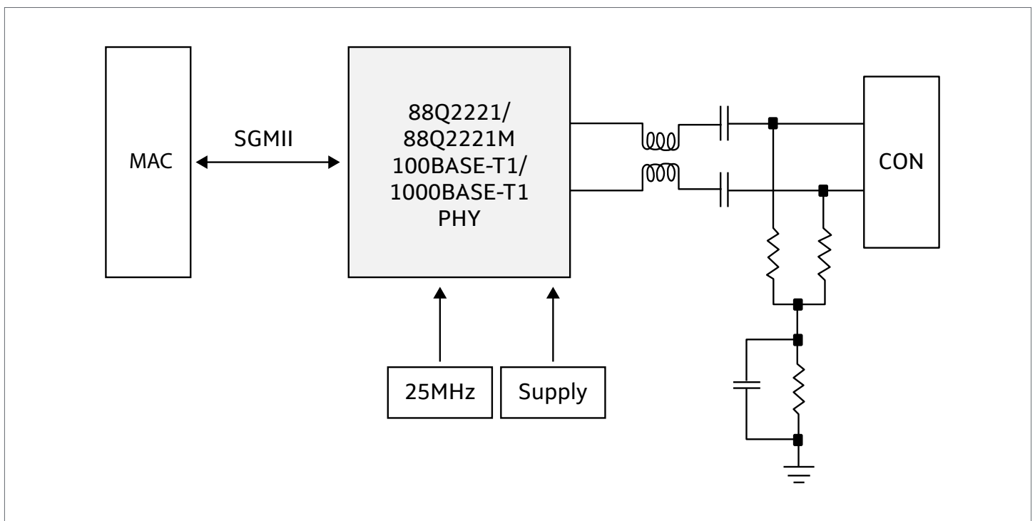
88Q222xM Block Diagram
