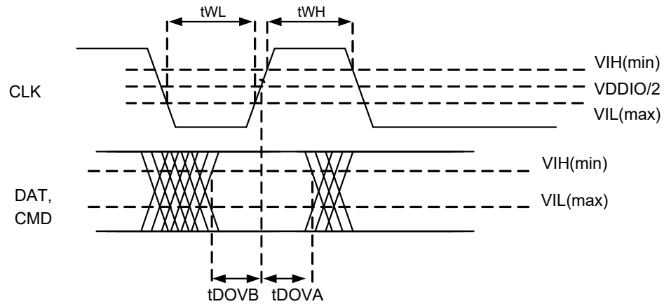
Figure 42: MMC High-Speed Host Input AC Timing Diagram
