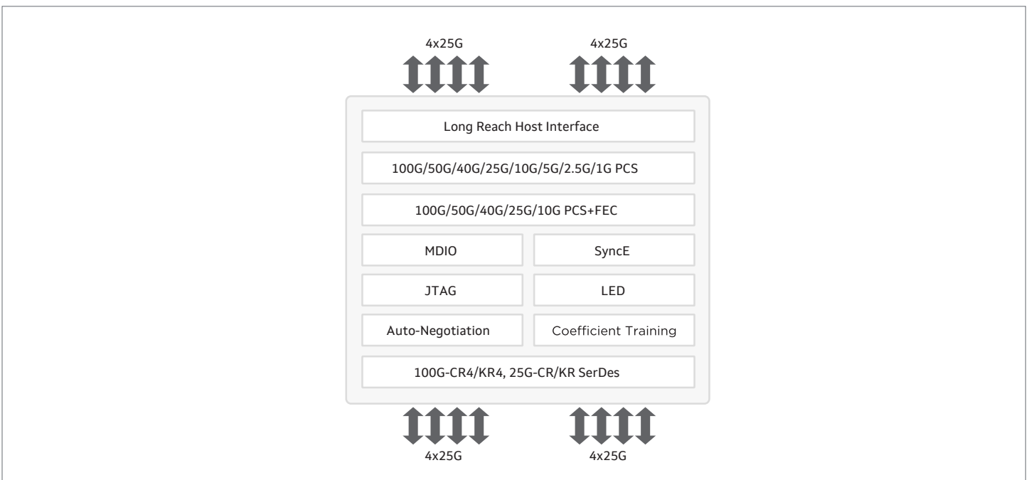
Marvell Alaska C 88X1523 Transceiver
