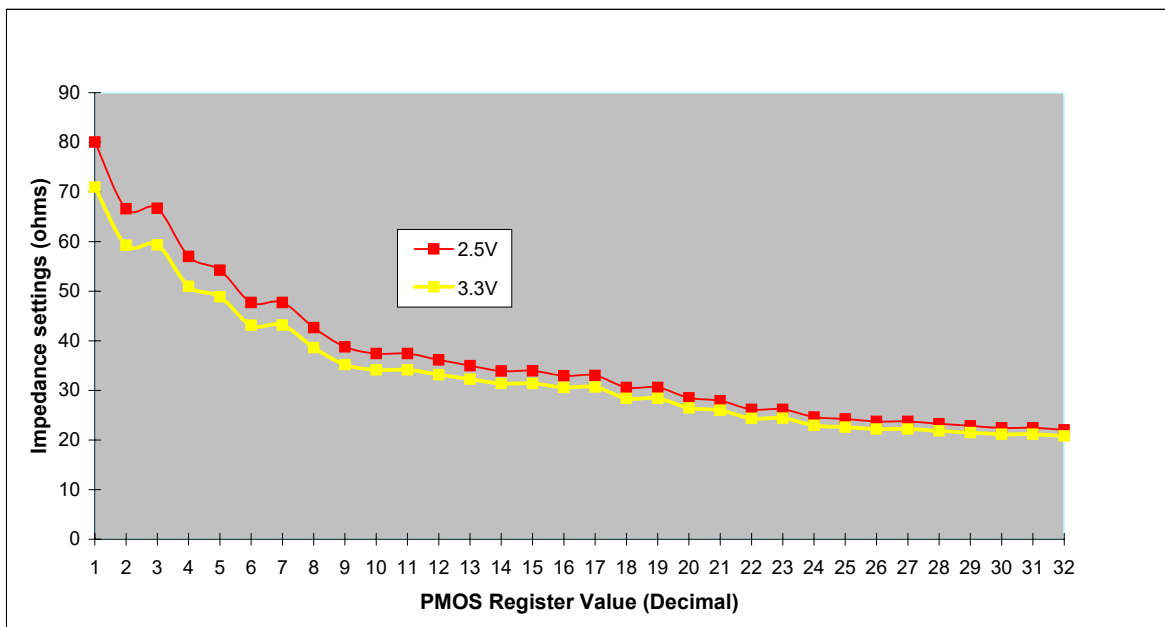
Figure 8: PMOS Output Impedance (1.8V, 2.5V) Trend Lines
