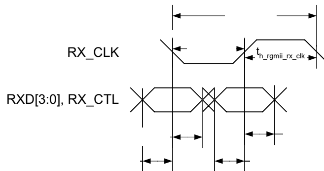
Figure 18: RGMII RX_CLK Delay Timing - Register 28.11:10 = 01 (add delay)
