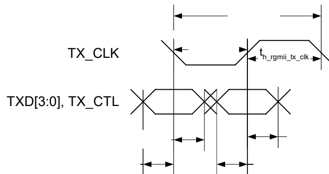
Figure 16: RGMII Transmit Timing
