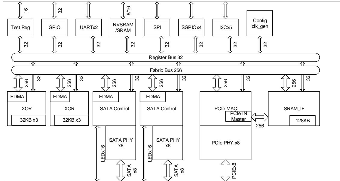
Figure 1-1 88SE1475 System Architecture
