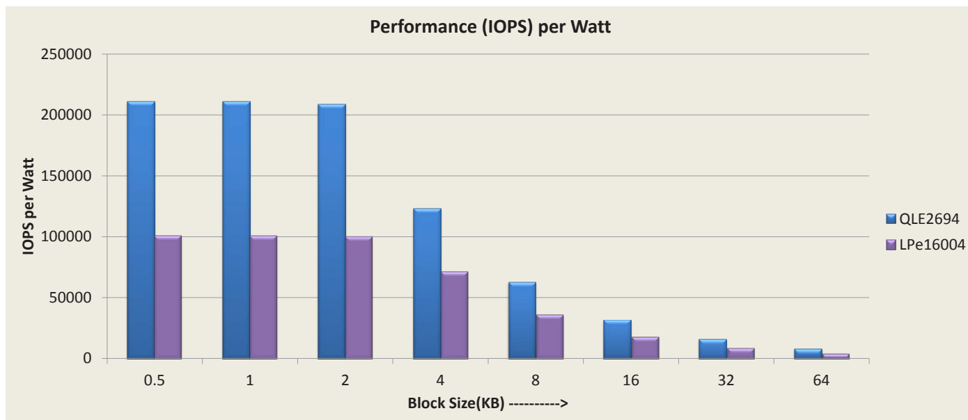
Figure 4. QLogic Adapters Deliver Twice the Transactional Performance per Watt
