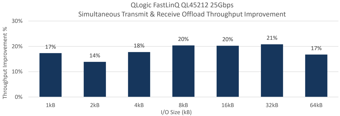
Figure 9. QLogic FastLinQ QL45212 25Gbps Simultaneous Transmit and Receive Offload Throughput Improvement
