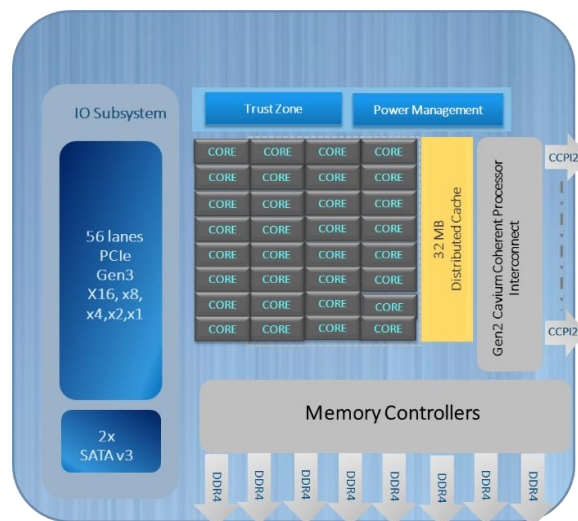
Figure1: High Level Block Diagram of Marvell ThunderX2
