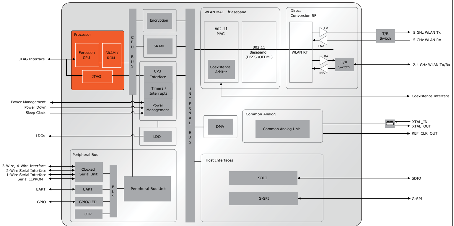
Fig 1. Avastar 88W8782 SoC Block Diagram
