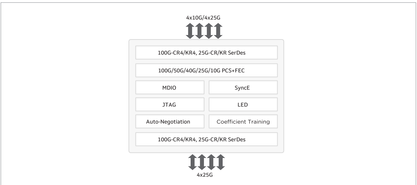
Marvell Alaska C 88X5113 Transceiver
