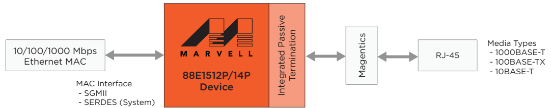
Figure 3: SGMII to Copper Application
