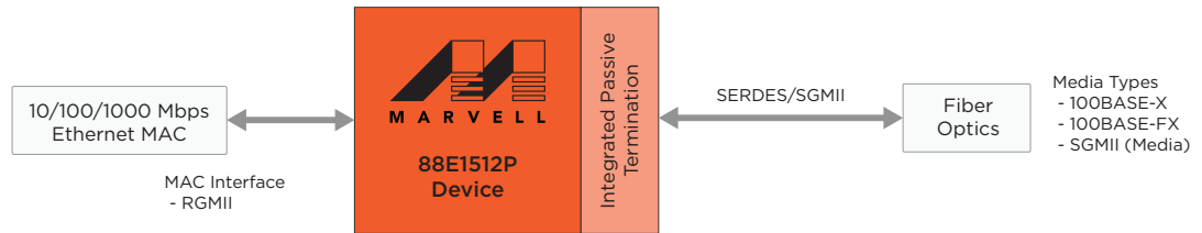
Figure 2: RGMII to Fiber/RGMII Application
