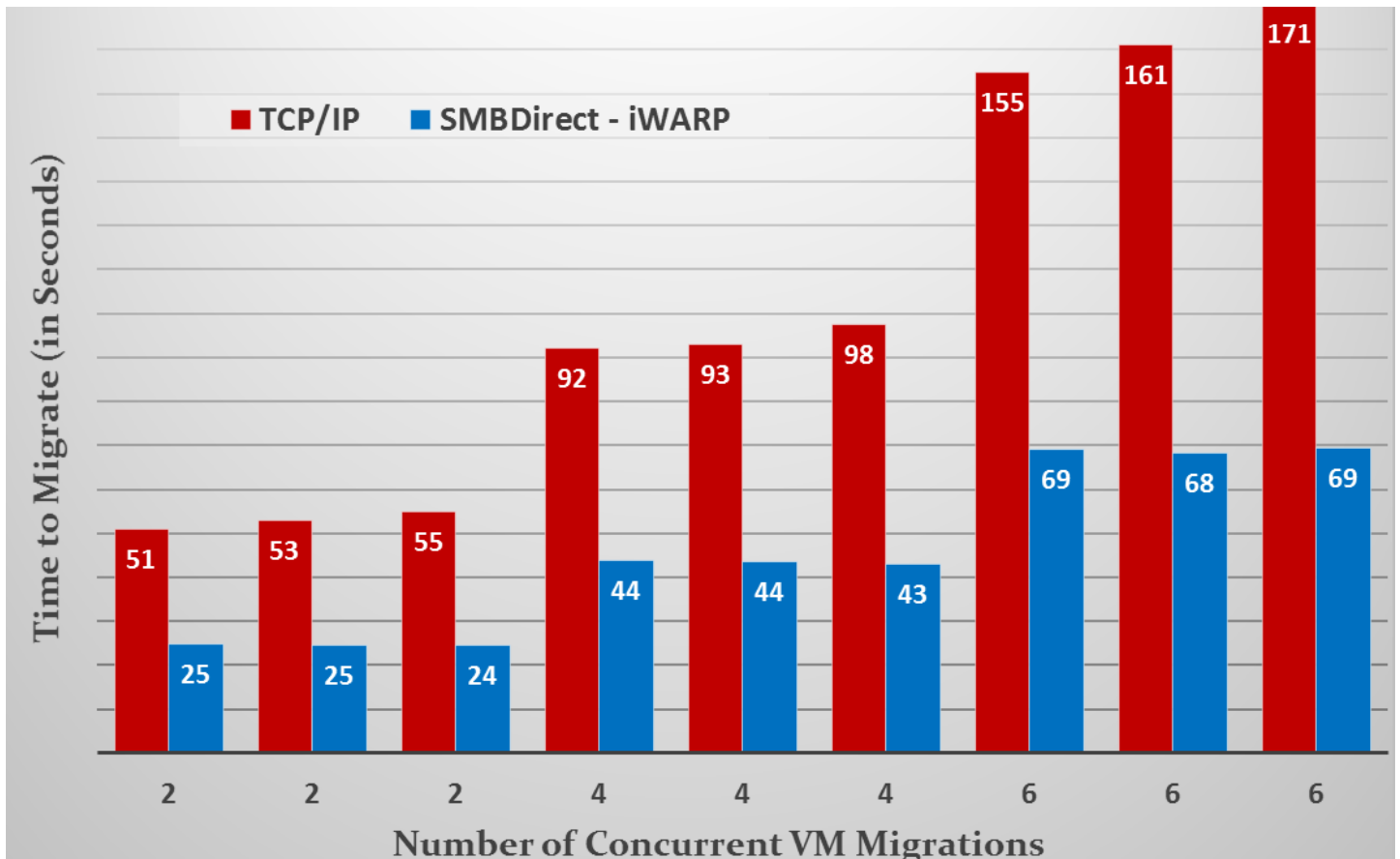
Figure 2. Live Migration: Windows Server 2016 with FastLinQ 41000 Series 25GbE Adapters
